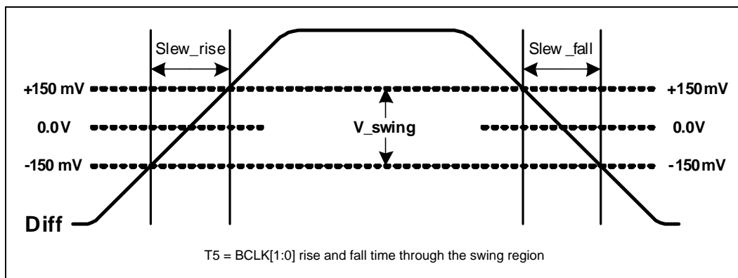
Figure 4. Measurement Points for Differential Clock Waveforms
