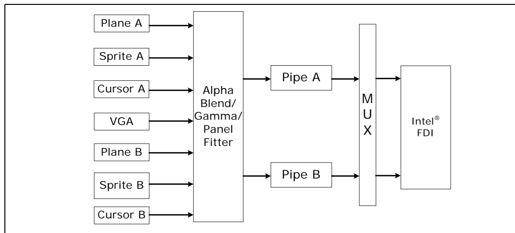
Figure 2-7. Processor Display Block Diagram
