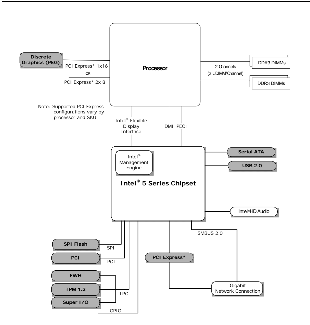
Figure 1-1. Intel® Core™ i5-600, i3-500 Desktop Processor Series and Intel® Pentium® Processor G6950 Platform Diagram
